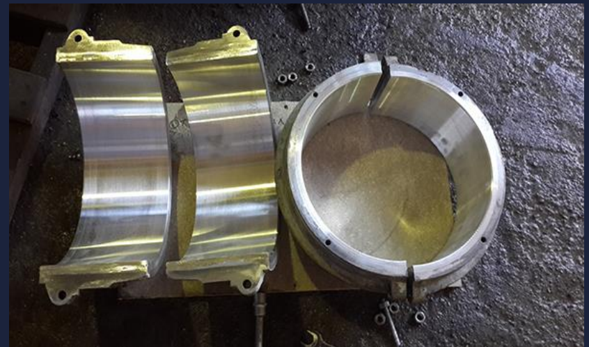
Renovated bearings with babbitt coating
