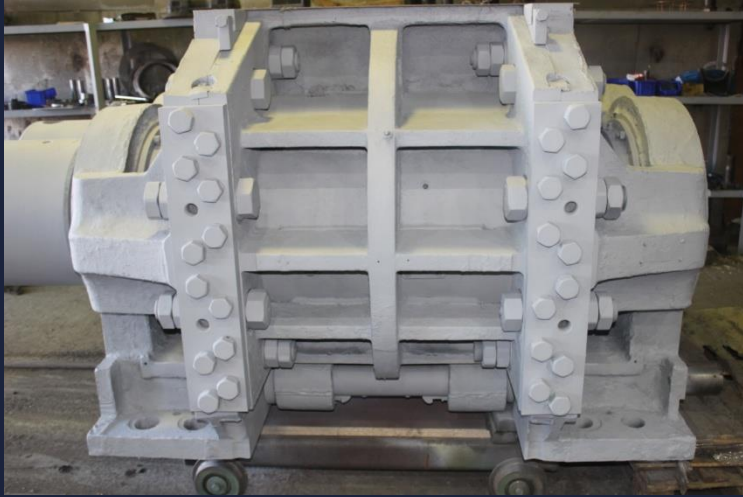
Building-up welding of semi-channel inner surface
